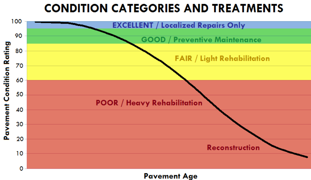
Figure 3: Pavement condition degradation and general treatment descriptions
